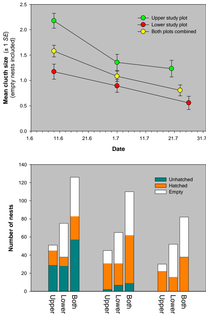
Figure 3.1.26 Seasonal variation in observed clutch size (top) and the parallel distribution of nests contents (bottom) of shags in the two study plots at Runde in 2007. Unhatched = egg(s) only; Hatched = at least one chick (some nests also contained 1-2 eggs); Empty = no eggs or chicks.
