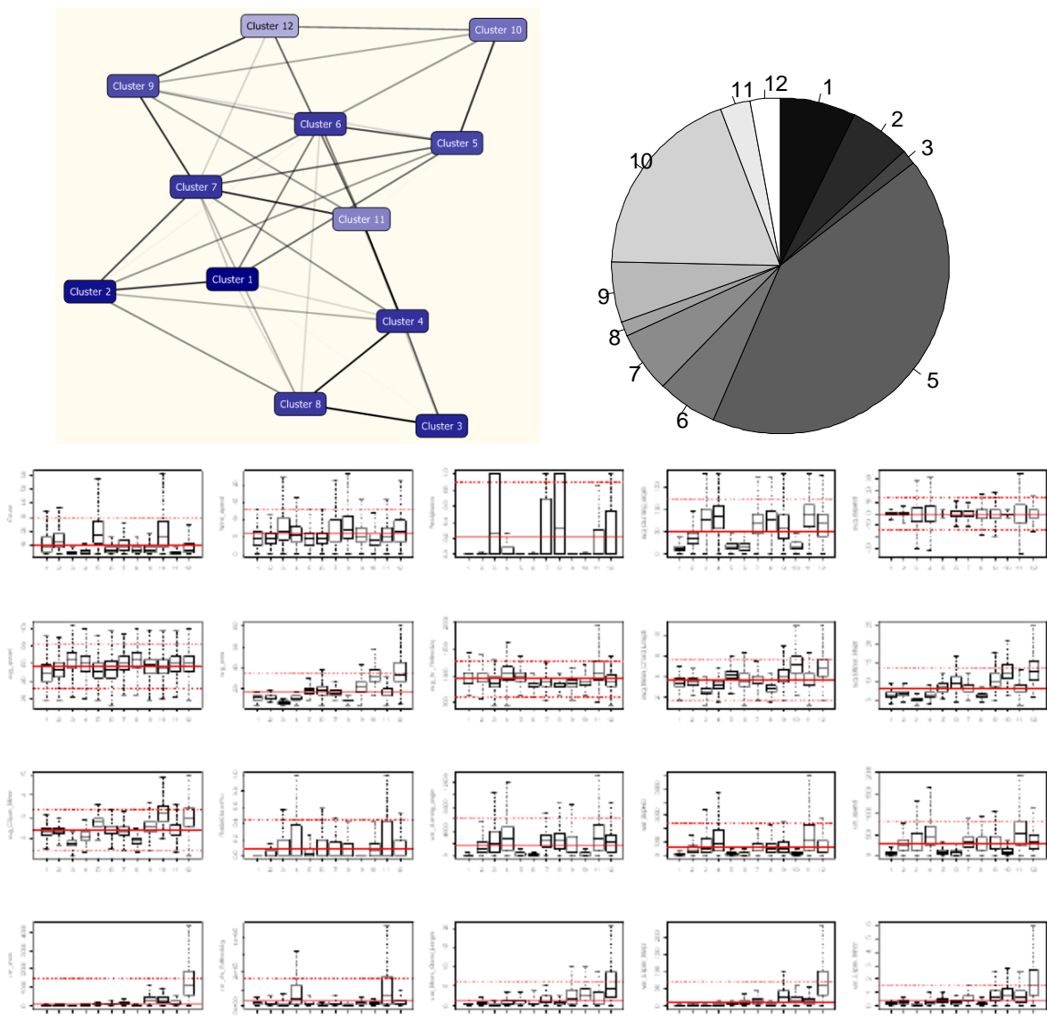
Figure 45. Exemplary results from the Microsoft SQL Server Data Mining Clustering technique based on a test database. The pie chart gives the distribution of the ground-truth tracks over the
