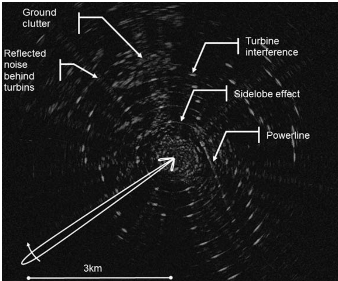
Figure 76. Radar-induced clutter in the Smøla wind-power plant area.
